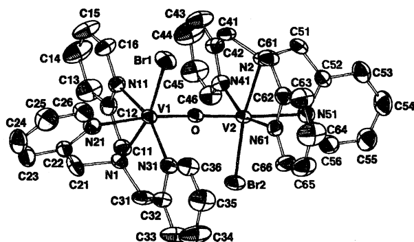
Fig. 6. Perspective view of [V_2(\mu-O)Br_2(tpa)_2]^{2+} .
