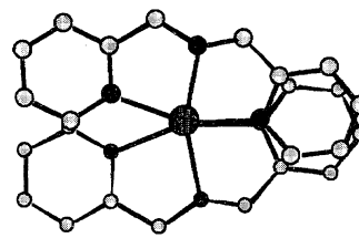
Fig. 7. View of [V_2(\mu-O)Br_2(tpa)_2]^{2+} from the direction of V...V axis. The methylpyridyl groups in the axial positions and bromo ligands are omitted for clarification.
